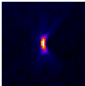
top left: PSF cross section of a commercial PS Check bead bottom left: PSF cross section of a Zebra Pen Mildliner particle scale: images are 8.13\mu\text{m} \times 8.13\mu\text{m} top right: intensity profiles across the centre of both
